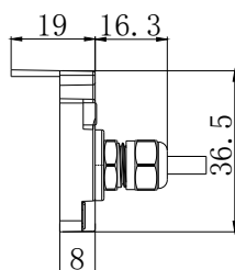
KTF1C: 防水接头式 Waterproof joint type
