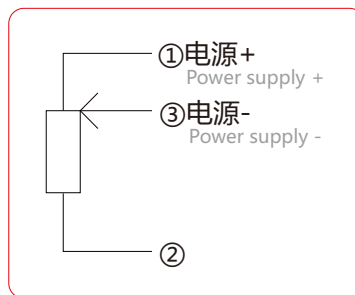
错误接线：图2 False wiring: Figure 2
