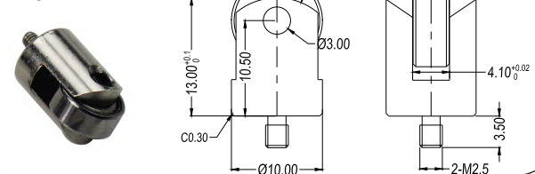
滑轮头 pulley block
