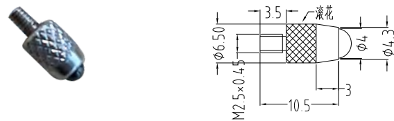
弧形尖头 curved tip
