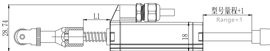
TR12滑轮头 TR12 Pulley head
