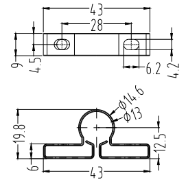
五金支架 Hardware bracket
