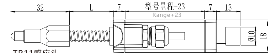
TR11感应头 TR11 Inductive head
