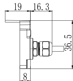
KTC11SC: 防水接头式 Waterproof joint
