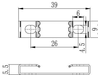
五金支架 Hardware bracket
