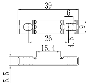
标配五金支架 Standard hardware support
