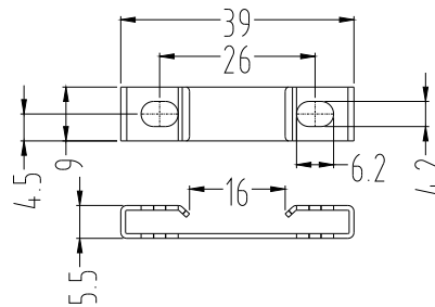
五金支架 Hardware bracket
