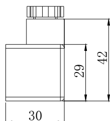
KTF1: 赫斯曼插头式(标配) Hersman plug (standard)
