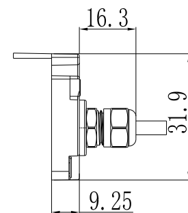
KTC11C/KTC1C/LWHC: 防水接头式 Waterproof joint
