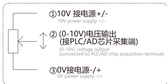
正确接线：图1 Correct wiring: Figure 1
