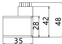
H2赫斯曼大插头 H2 Hermann large plug
