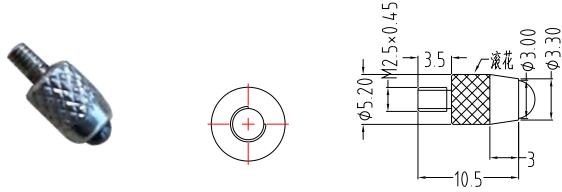
氮化硅陶瓷球头 Silicon nitride ceramic ball
